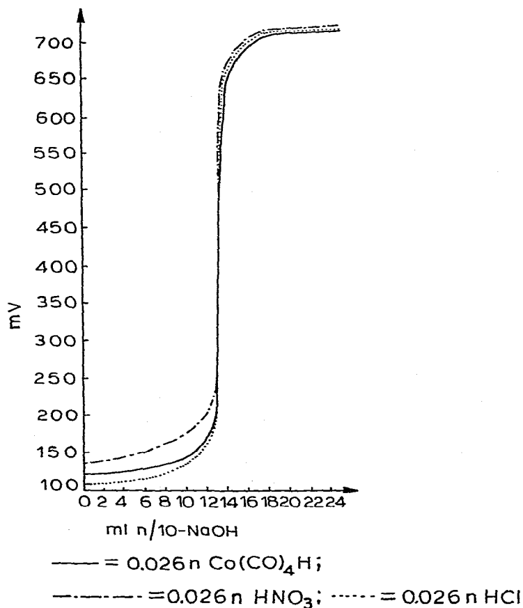
Fig.17. Potentiometric titration curve of \text{HCo}(\text{CO})_4 in methanol ( 0^\circ\text{C} ).
